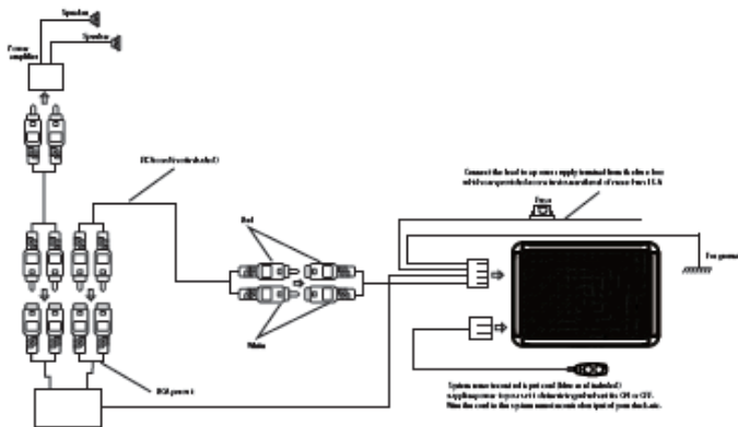
Wiring Example 2 (RCA Input system)
