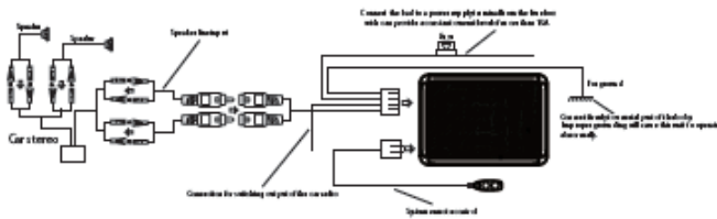
Wiring Example 1 (Speaker line input system)
